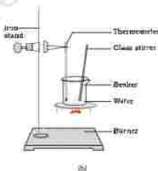
Fig. 1.6: (a) Conversion of ice to water, (b) conversion of water to water vapour
