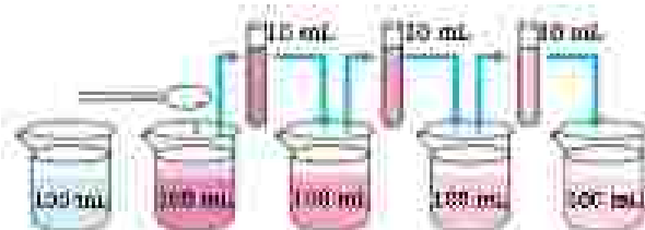
Fig. 1.2: Estimating how small are the particles of matter. With every dilution, though, the colour becomes lighter, & it still remains.
