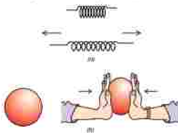
Fig. 9.2: (a) A spring expands on application of force; (b) A spherical rubber ball becomes oblong on the application of force on it.
