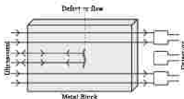
Fig 12.16: Ultrasound is reflected back from the defective location inside a metal block.
