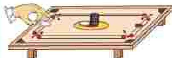
Fig. 9.6: Only the bottom coin at the bottom of a pile is removed when a fast moving circular coin (or striker) hits it.
