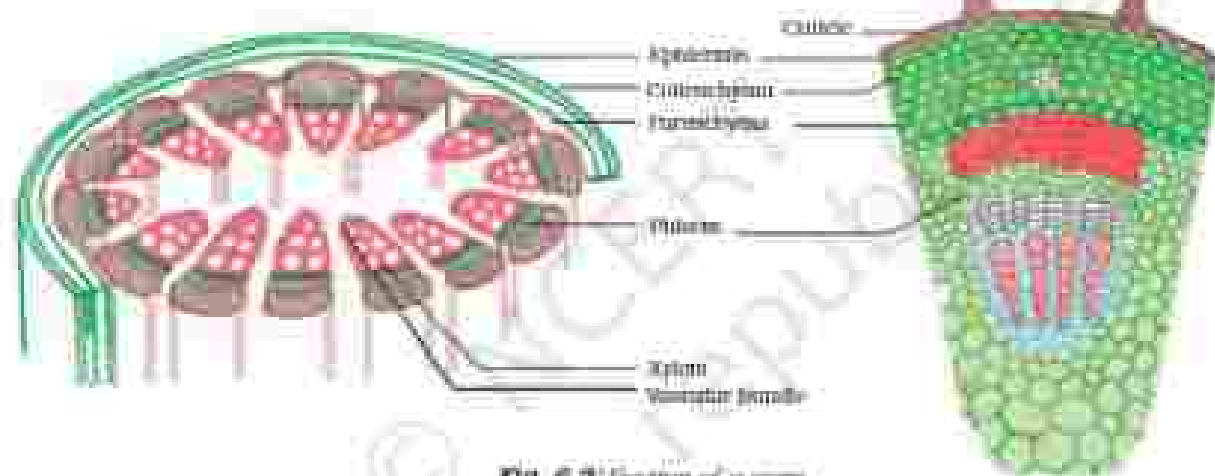
Fig. 6.3: Section of a stem
