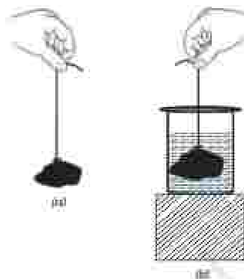
Fig. 10.6: (a) Observe the elongation of the rubber string due to the weight of a piece of stone suspended from it or (b) The elongation decreases as the stone is immersed in water.
