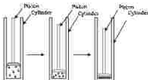
Fig. 1.8: By applying pressure, particles of matter can be brought closer together.
