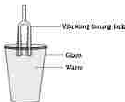
Fig. 12.3: Look the prongs of the vibrating tuning fork dipped in water.
